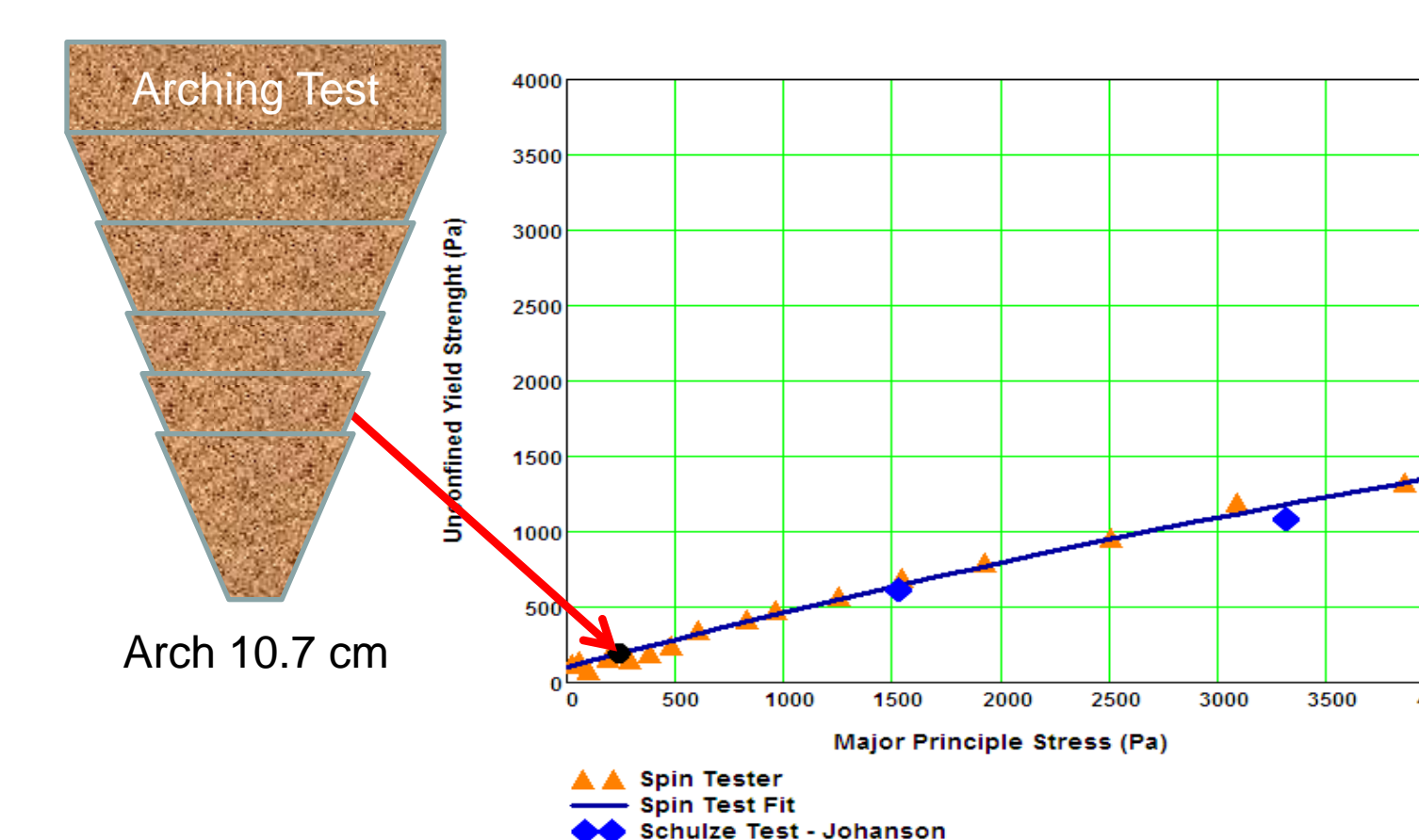
Figure 5. Comparison of the lower stress level unconfined yield strength of Argo corn starch measured with the Schulze direct shear method and the new test technique (SSSpinTester)
