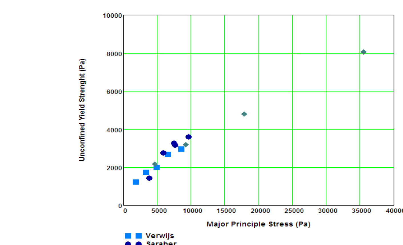
Figure 1. Comparison of BCR Limestone data generated from three different studies
