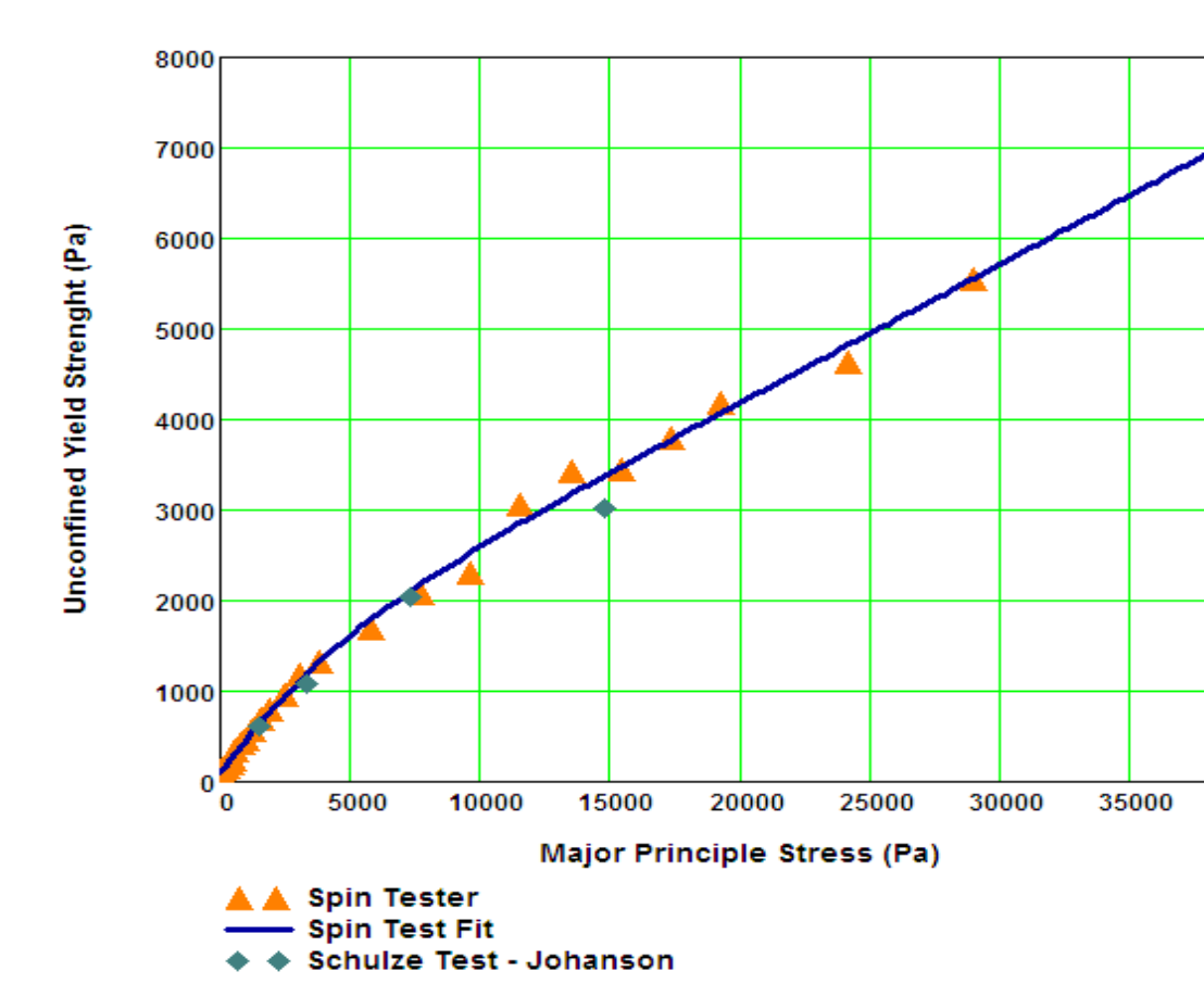
Figure 4. Comparison of the unconfined yield strength of Argo cornstarch measured with the Schulze direct shear method and the new test technique (SSSpinTester)
