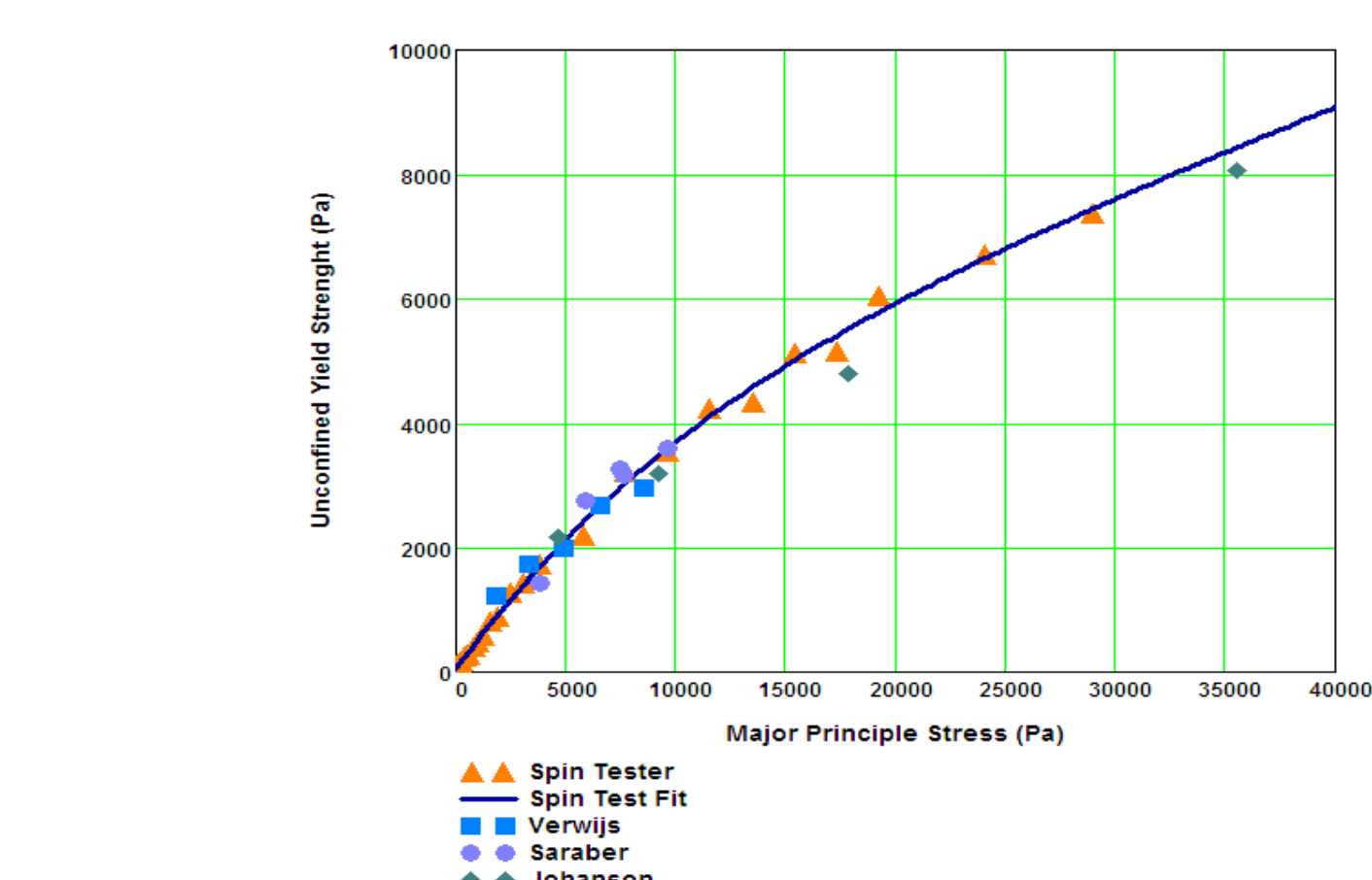
Figure 2. Comparison of BCR limestone data generated from three different studies and new test technique (SSSpinTester)
